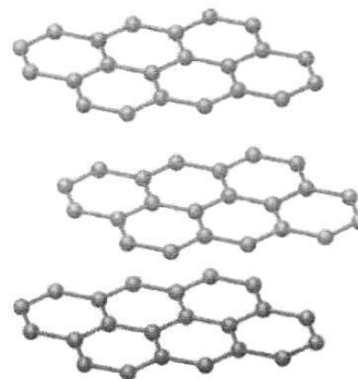
Fig. 3.4 Structure of graphite
