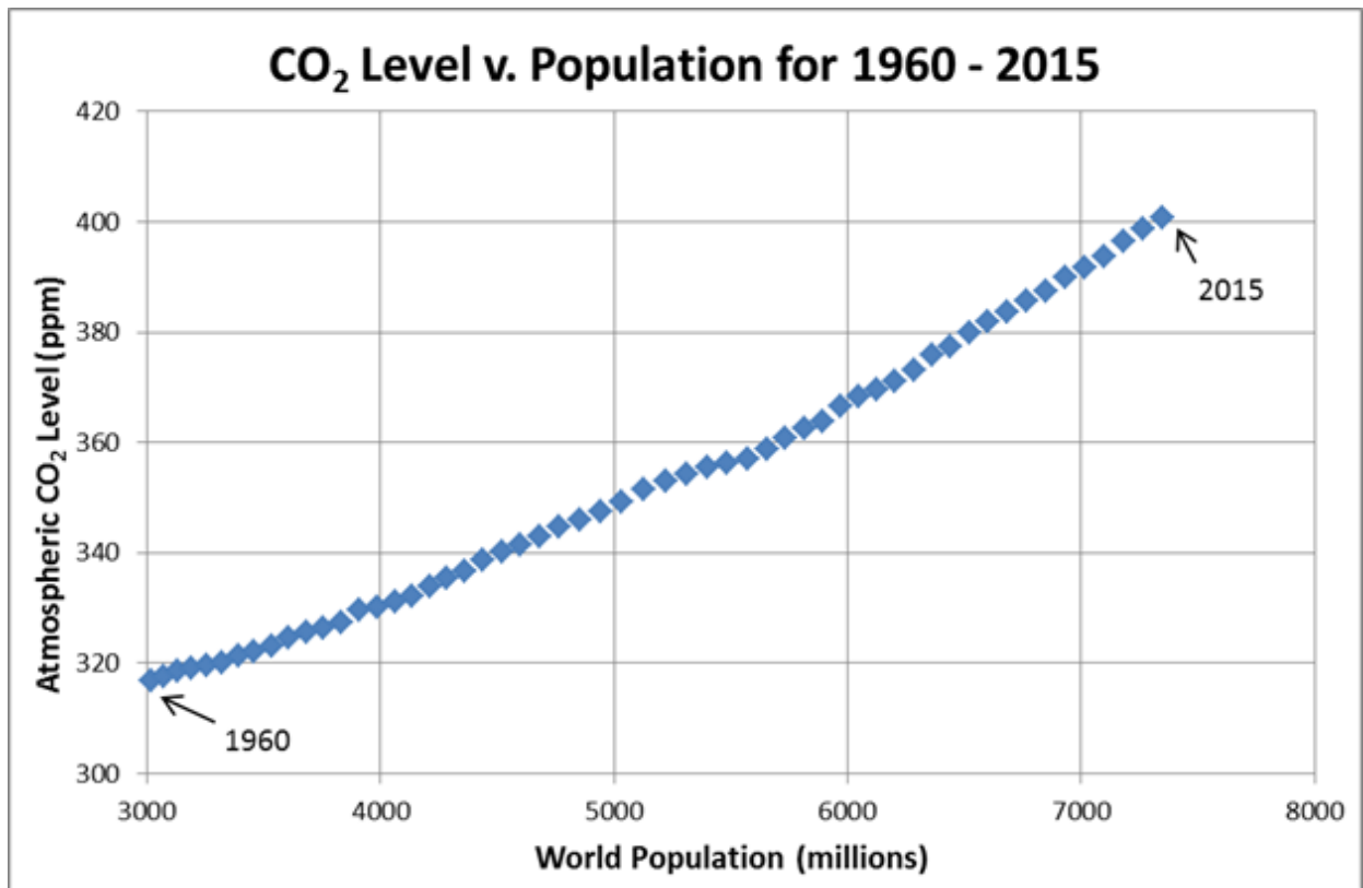
Fig. 5: CO 2 level vs world population for 1960-2015
