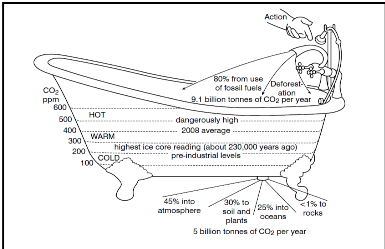
Fig. 4: An illustration outlining the input and output of CO 2
