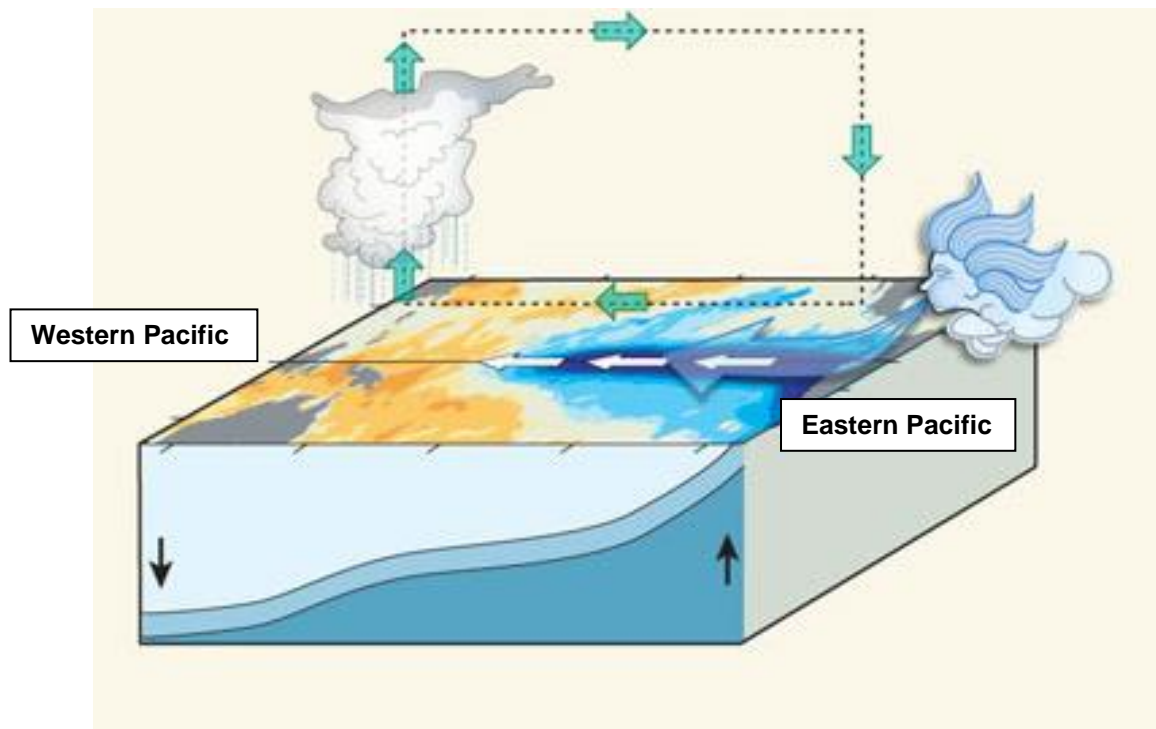
Fig. 8A: Normal Conditions (walker circulation)
