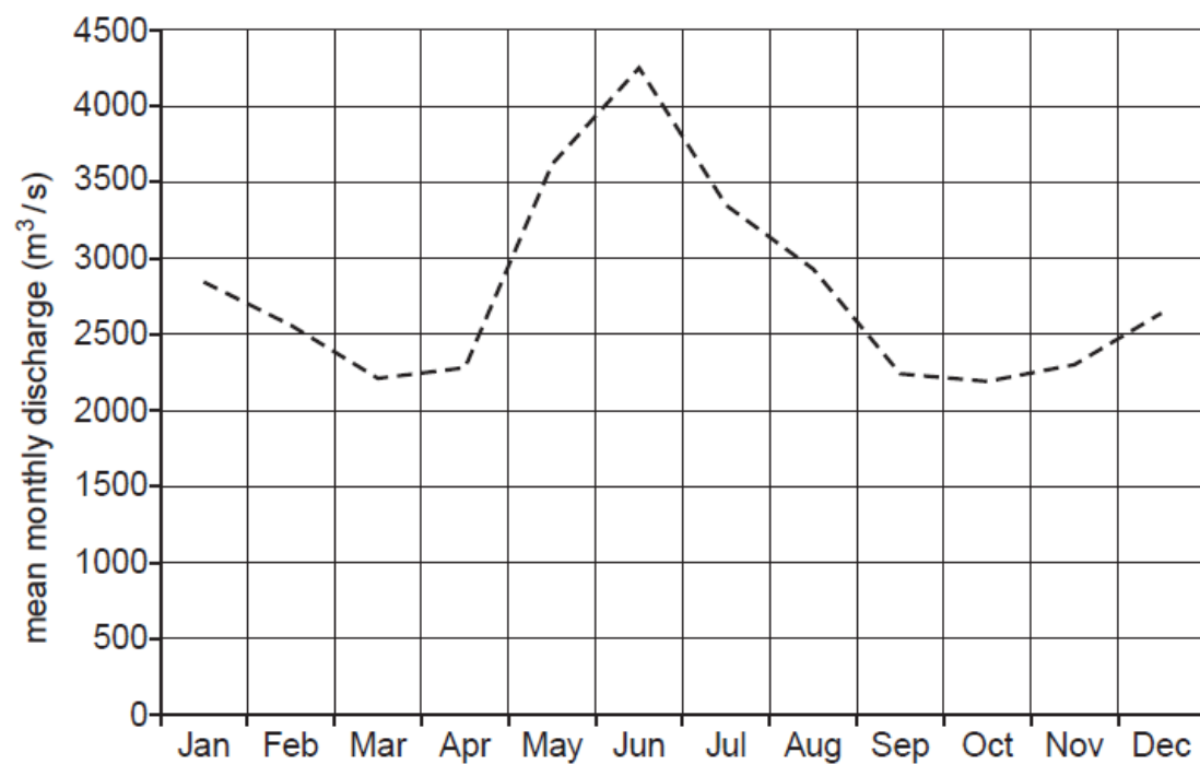
Fig. 7: Annual Hydrograph for the Columbia River in Canada
