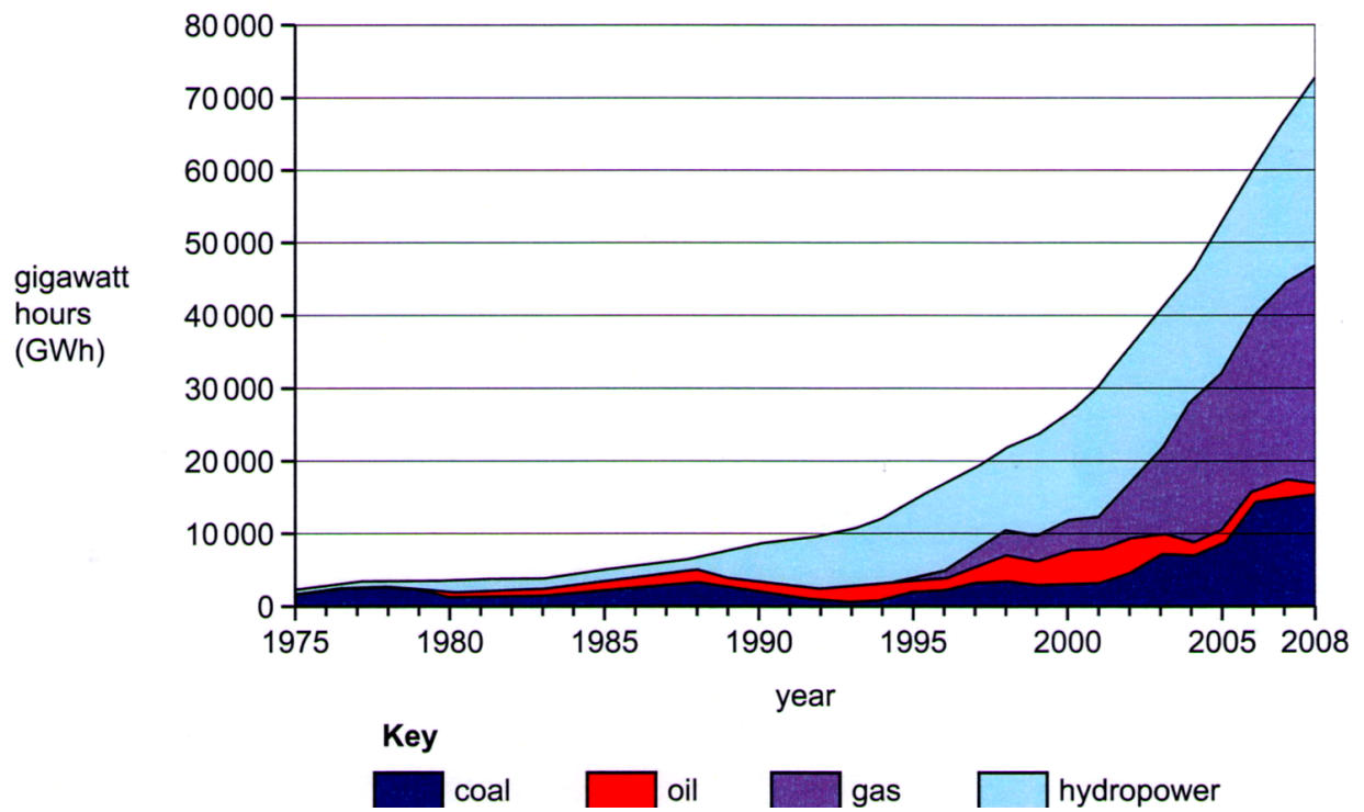
Electricity generation in Vietnam by fuel type, 1975-2008
