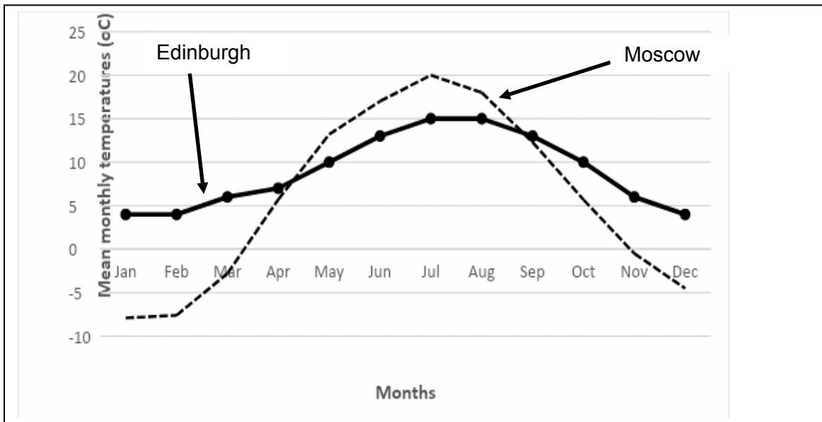
Fig. 3.2 for Question 3. Mean monthly temperature of two cities.
