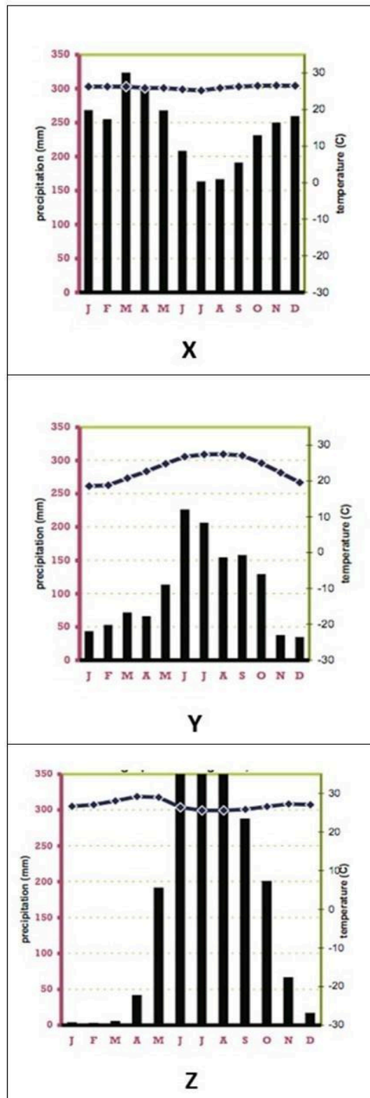
Fig. 2.1 for Question 2 Climographs of Places X, Y, and Z
